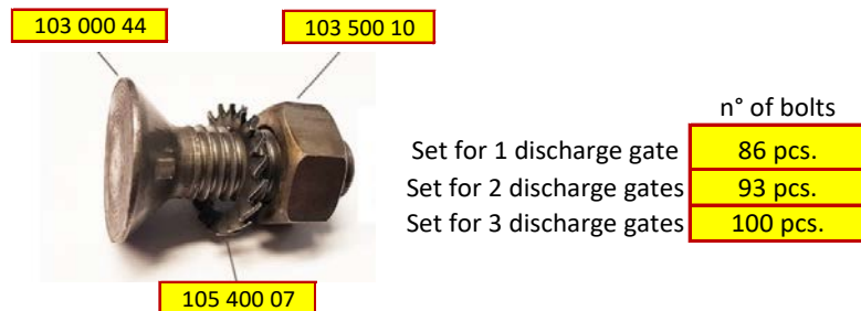
Set of fixing bolts for bottom plates
