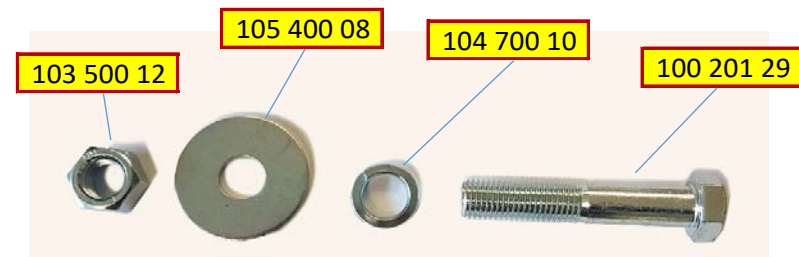
Bolt for rubber shovels fixing
