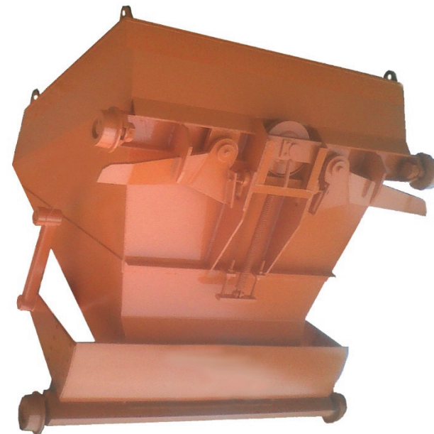
Skip hoist bucket
