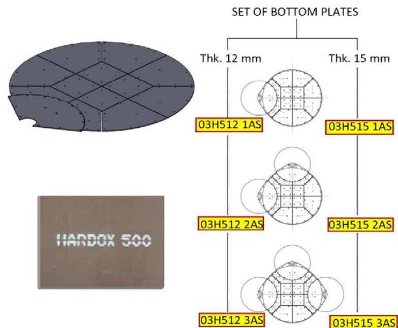
Set of bottom plates
