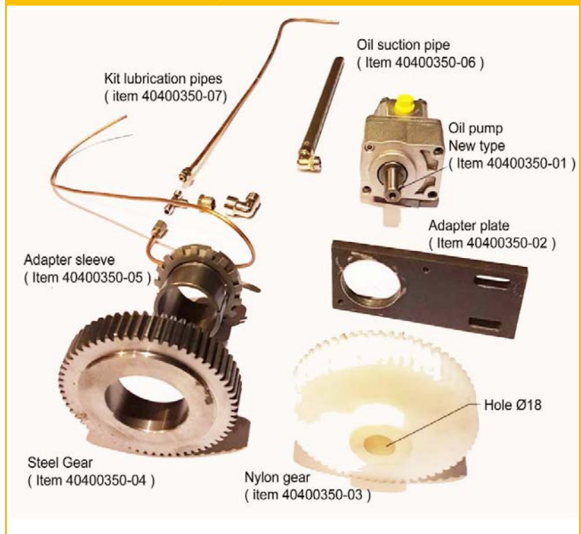
Oil pump set
