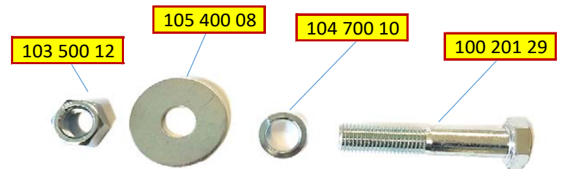
Bolt for rubber shovels fixing
