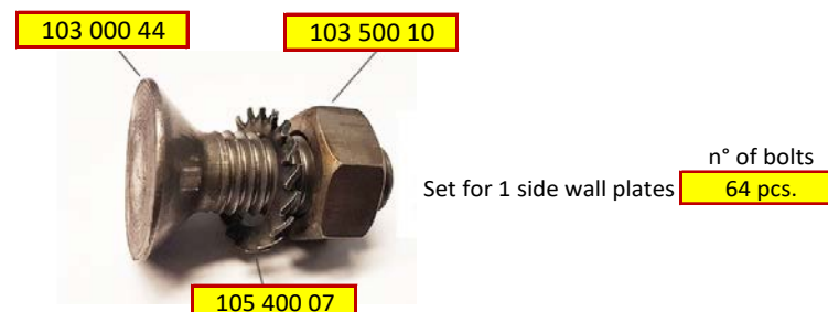
Set of fixing bolts for side wall plates
