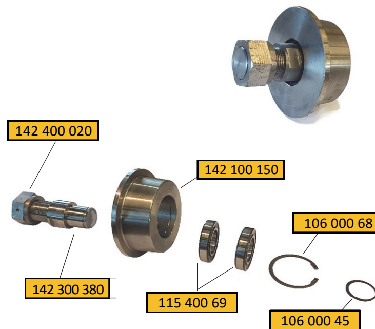
Skip hoist wheel
