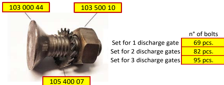
Set of fixing bolts for bottom plates
